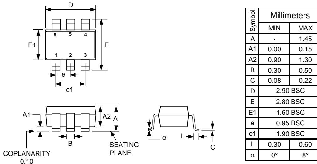
Figure 10.1: Physical dimensions, 6-lead SOT-23 package
