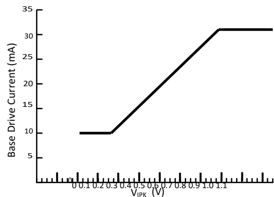
Figure 9.5: Base Drive Current vs. V_{IPK}
