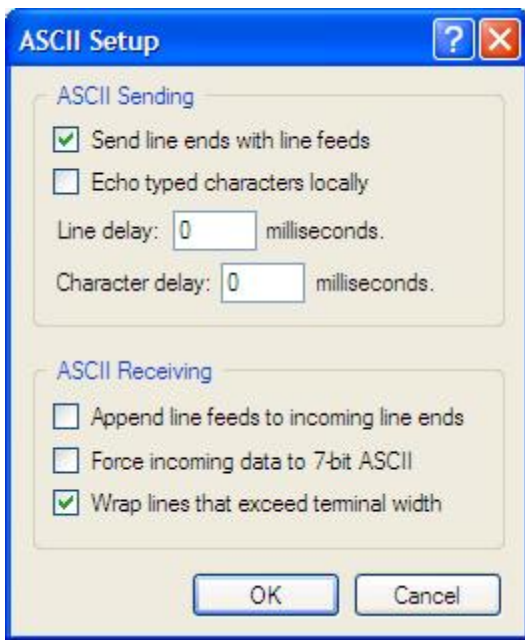
Figure 2: HyperTerminal setup
